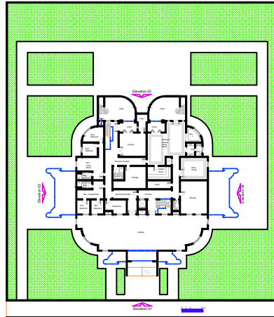
Lower Floor Plan A = 559,69 m 2
