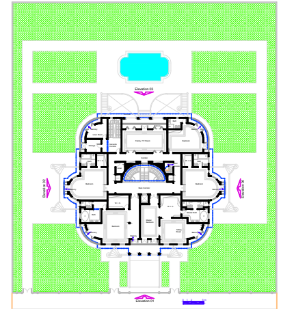
Second Floor Plan A = 537,70 m 2
