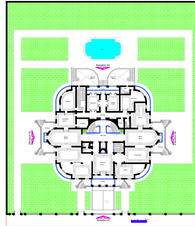
First Floor Plan A = 562,10 m 2
