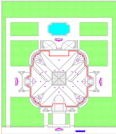
Roof Plan
